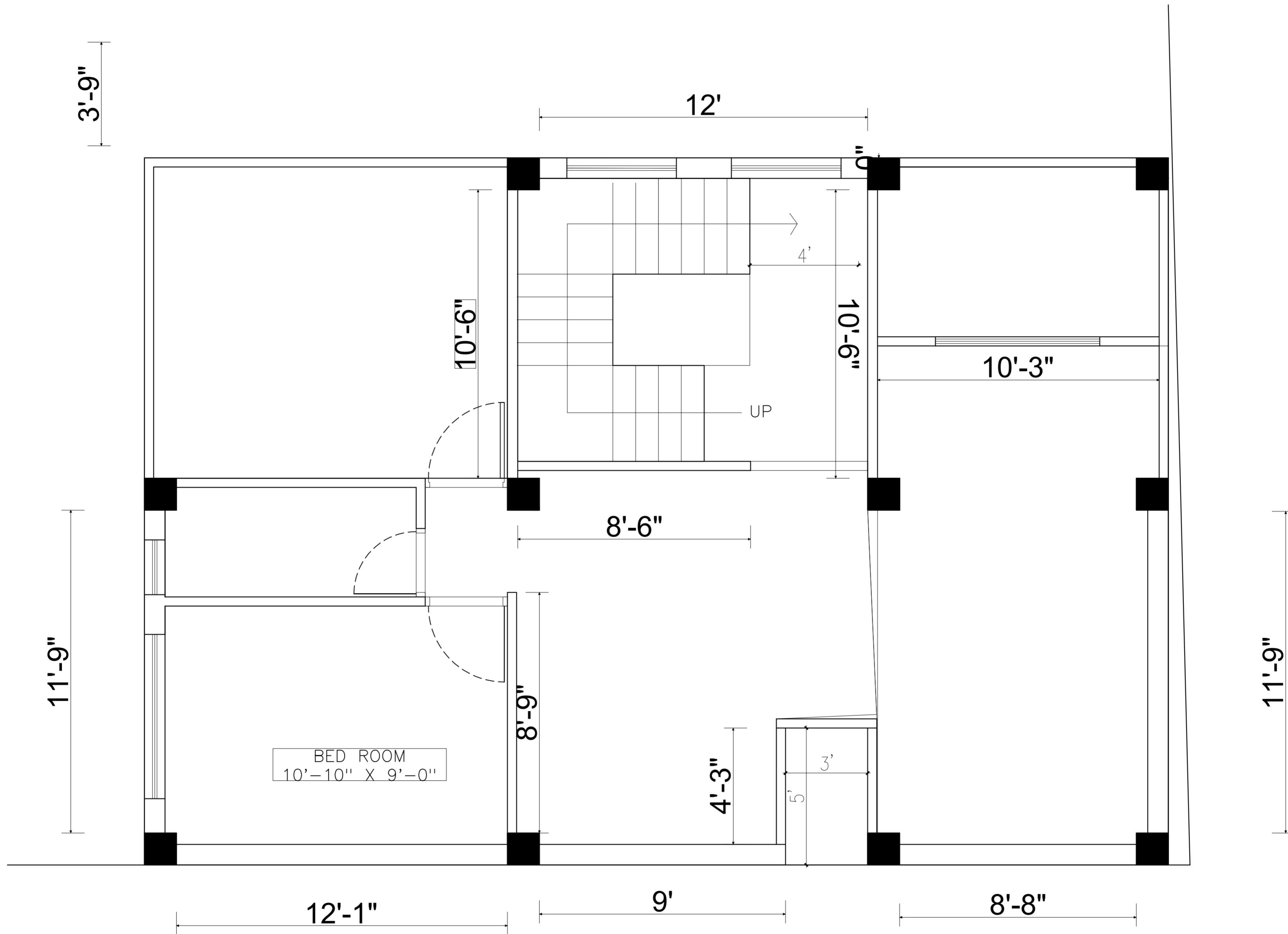
TOP FLOOR PLAN TOP FLOOR AREA:- 955.00 SQ.FT TOTAL AREA:-1372.00 SQ.FT.
